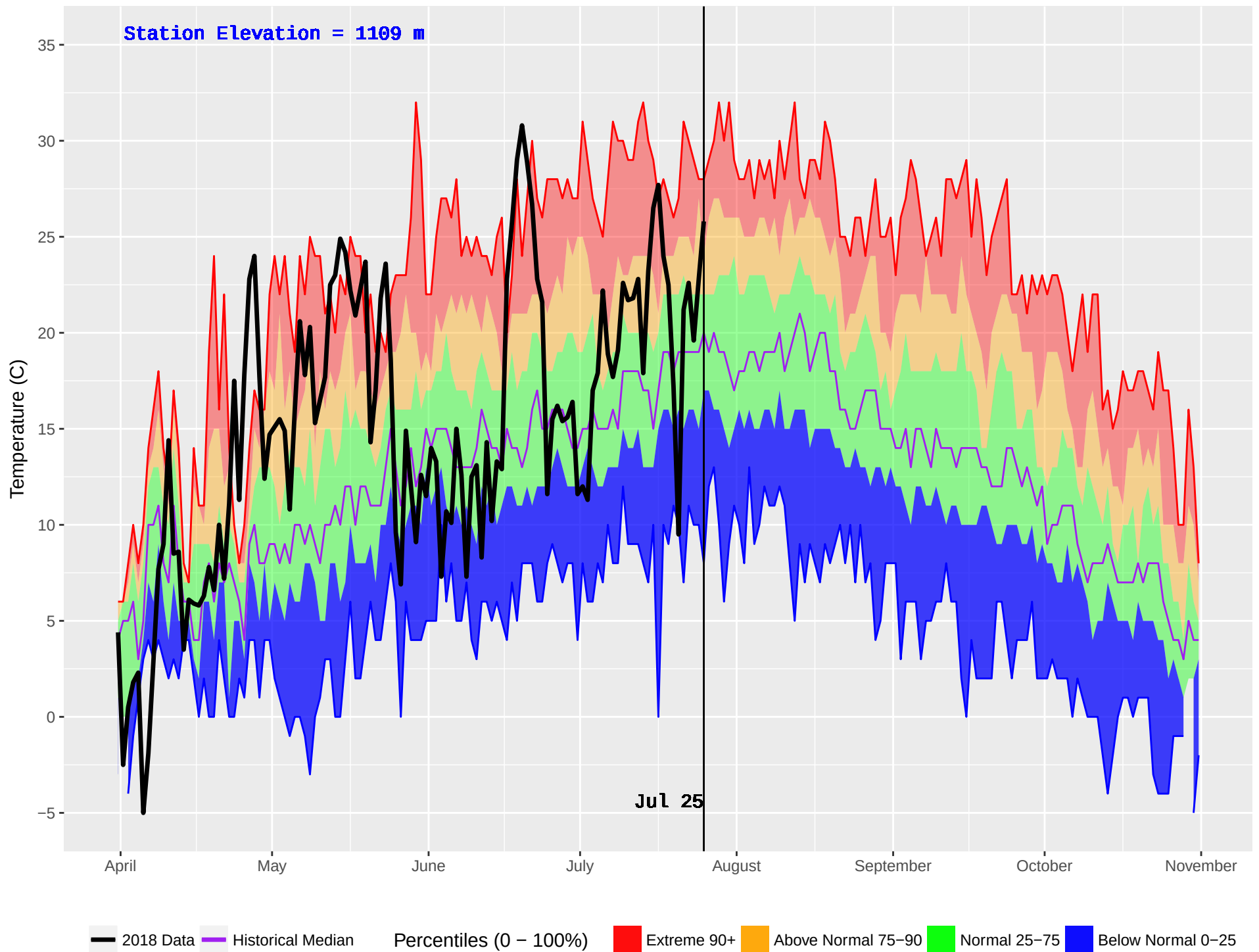
MOOSE LAKE (165) : Historical (1980–2016) and Current (2018) Noon Temperature
