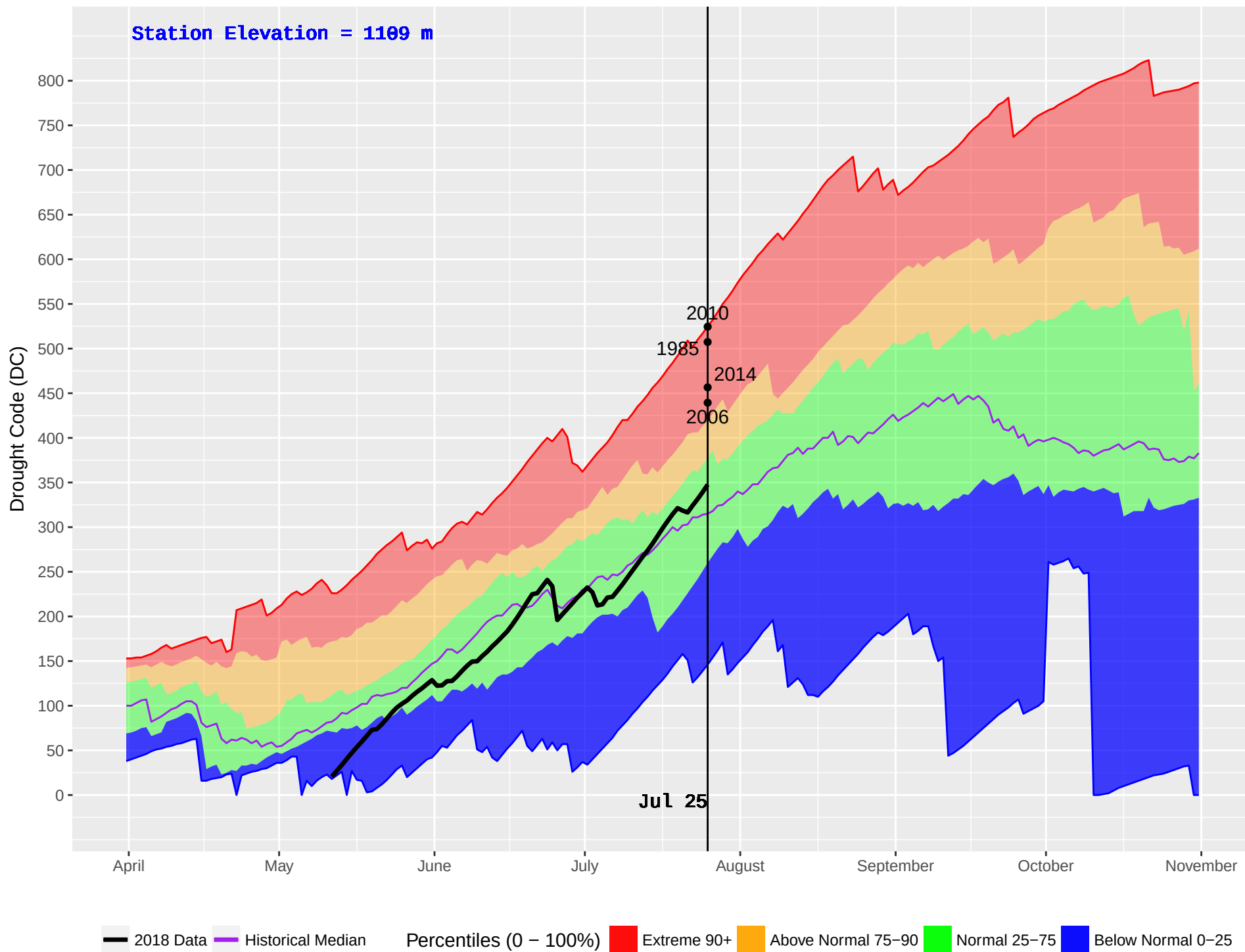
MOOSE LAKE (165) : Historical (1980–2016) and Current (2018) Noon Drought Code (DC)
