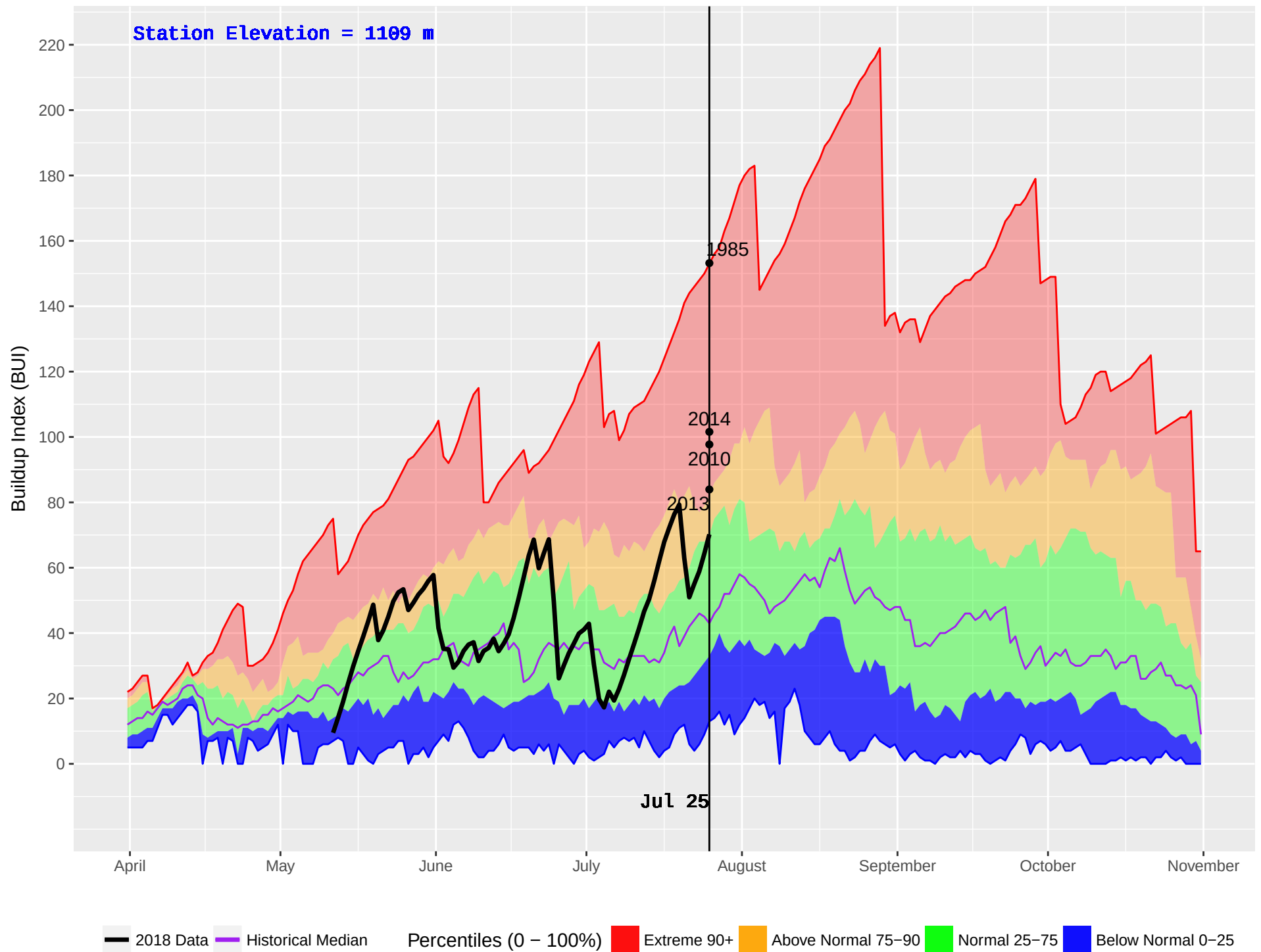
MOOSE LAKE (165) : Historical (1980–2016) and Current (2018) Noon Buildup Index (BUI)
